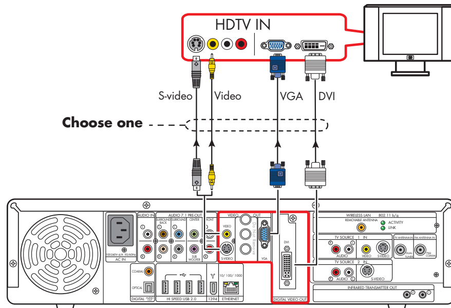
Video out to high-definition capable HDTV
